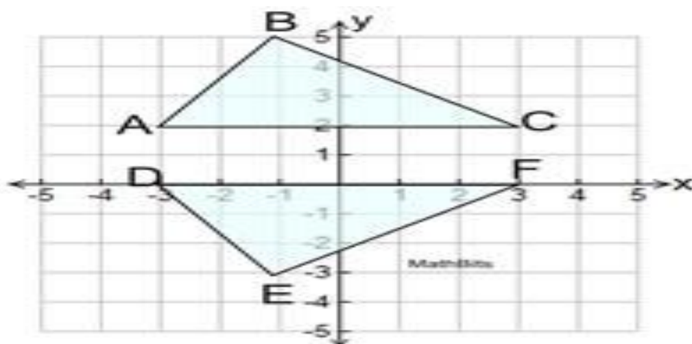
Figure 15. Symmetry demonstration
