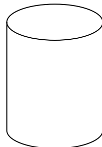
Cylinder
