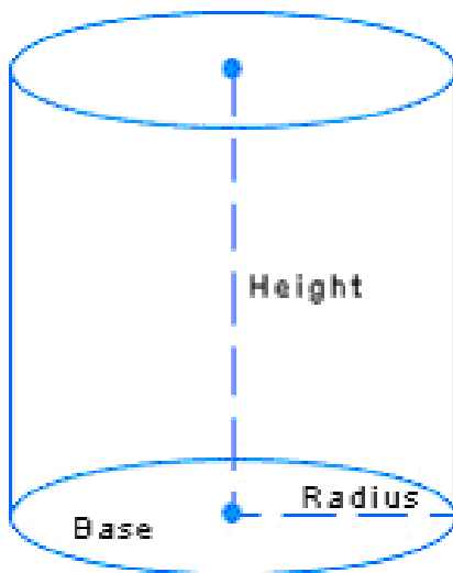
Figure 6. Cylinder
