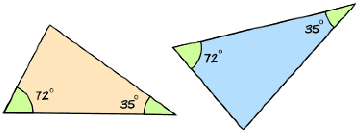
Figure 16. Congruent figures
